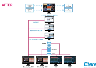
(IP Playout with IP Multiviewer )
