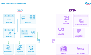
Etere AVID Integration Diagram
