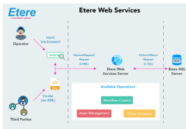
Web Services Diagram
