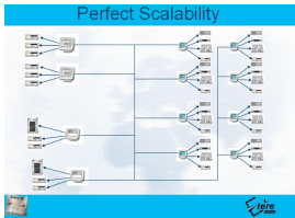
Perfect Scalability
