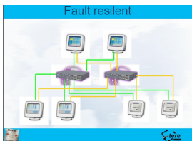
Fault Resilient
