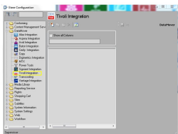
Tivoli Integration
