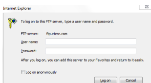
FTP Upload
