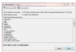
The GUI
