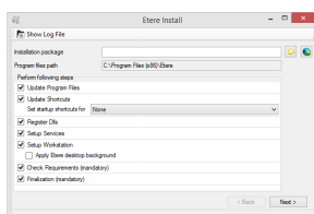
Ftere GUI
