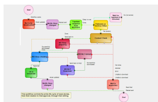
Nunzio workflow
