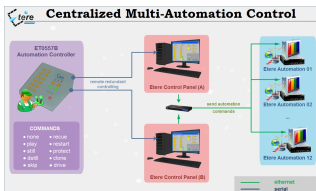
Etere Control Panel Flowchart
