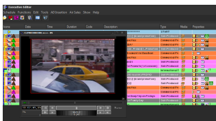
Scheduling GUI
